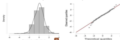
Diagram 1. Residuals vs. Histogram
