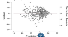
Diagram 3. Residuals vs. Predicted
