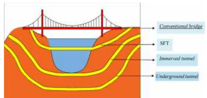
Figure 1. Illustration of water crossing comparison (Source: ITA/AITES,2006)
