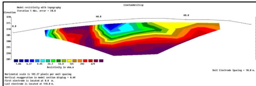
Gambar 5. Penampang 2D Lintasan 3
