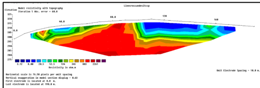
Gambar 3. Penampang 2D Lintasan 1
