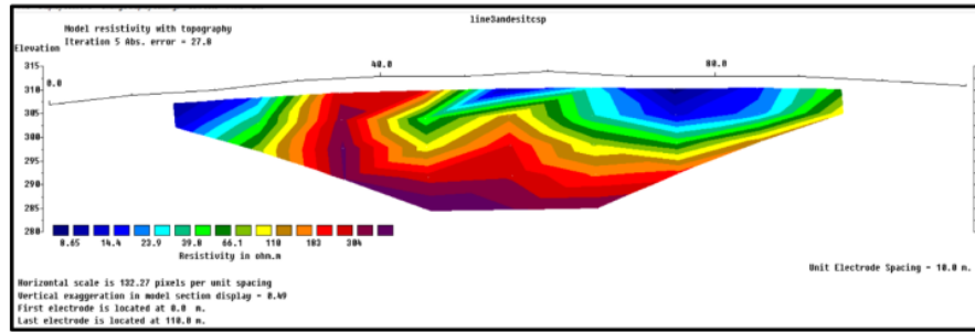
Gambar 6. Penampang 2D Lintasan 4
