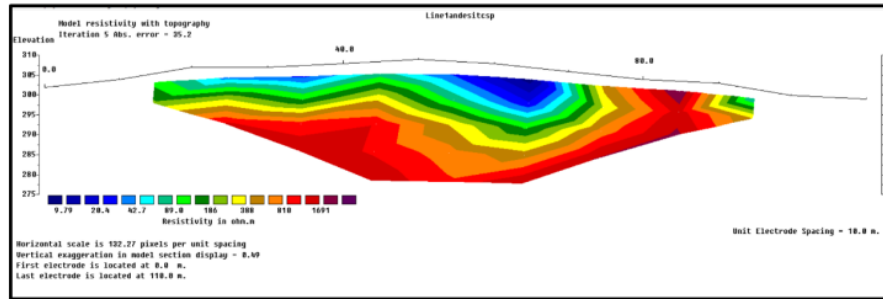
Gambar 4. Penampang 2D Lintasan 2
