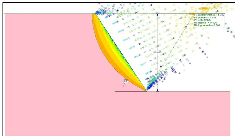
Gambar 5. Hasil Analisa Single Slope (Olahan Penulis, 2025)
