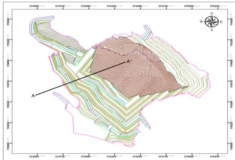
Gambar 2. Design Pit with Line Section (Olahan Penulis, 2025)
