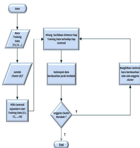
Gambar 1. Flowchart K-means [2]
