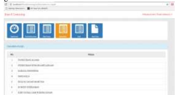
Gambar 3.5 Data Matakuliah
