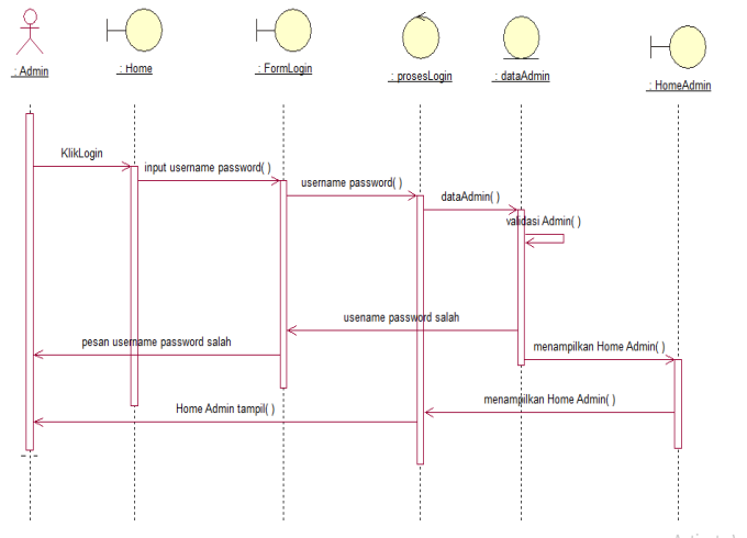
Gambar. 5. Sequence Diagram Proses login Admin
