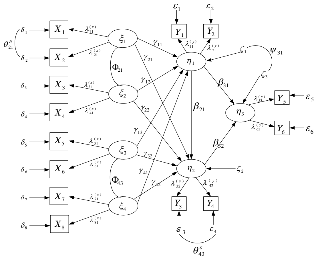
Gambar 1. Model Diagram Path LISREL
